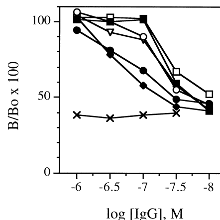
Fig. 2. Aah I neutralising capacity of anti-Aah I mAbs. Binding of Aah I ( 6.3 \times 10^{-8} M) to rat brain synaptosomes, in the presence of [ ^{125} I]Aah II ( 1.5 \times 10^{-10} M), was inhibited by preincubation with various concentrations of IgG from mAbs. Anti-Aah I mAbs inhibited the competitive binding between Aah I and [ ^{125} I]Aah II at the common receptor. B and Bo represent the reactivity measured in the presence (B) or absence (Bo) of mAb 9C2 (■), 2G3 (●), 10A10 (○), 10E6 (◆), 7D3 (□) and 5B5 (▽). BALB/c preimmune IgG was used as a control (X).
